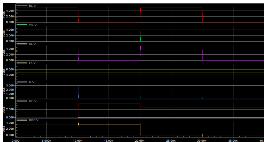
Fig. 10. Output Waveform of Dynamic Power Gated TG SRAM
