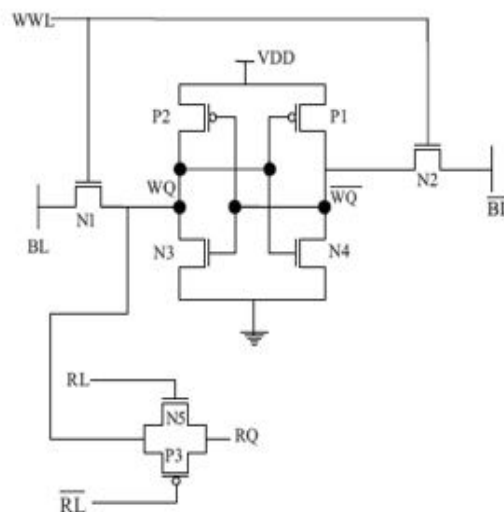
Fig. 2. Transmission Gate Based 8T SRAM
