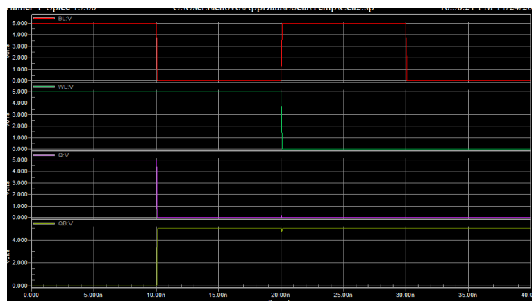
Fig. 5. Output Waveform of 6T SRAM cell
