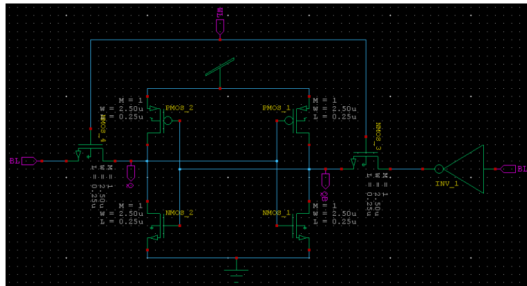
Fig. 4. Schematic Diagram of 6T SRAM cell
